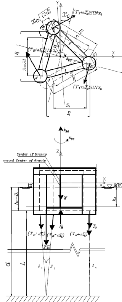
Fig. 6 The Yaw displacement in a triangular TLP
