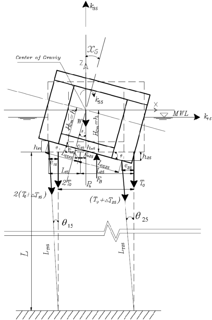
Fig. 5 The Pitch displacement in a triangular TLP
