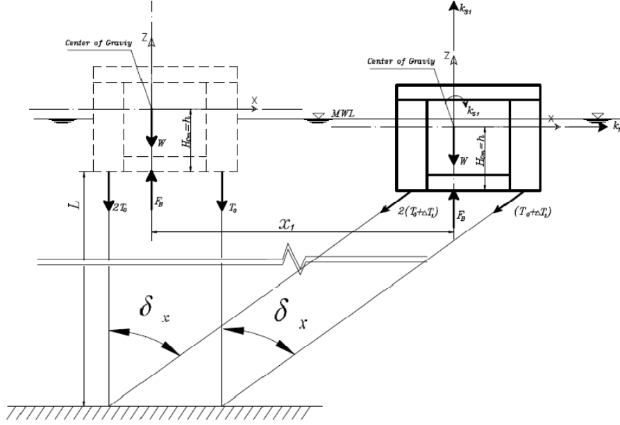
Fig. 2 The Surge displacement in a triangular TLP
