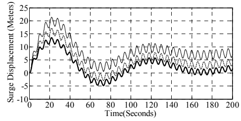
(a) wave period = 6 sec
