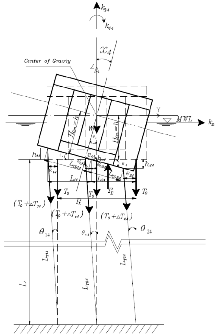
Fig. 4 The Roll displacement in a triangular TLP
