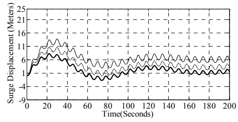
(b) wave period = 8 sec
