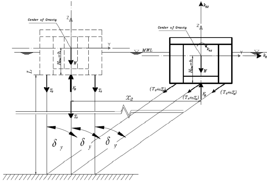
Fig. 3 The Sway displacement in a triangular TLP
