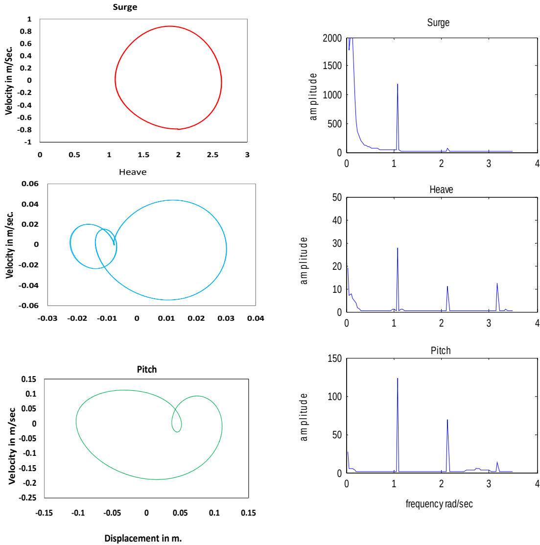
Fig. 10 Phase plane and response spectrum for wave period= 8 sec. and height = 8.0 m
