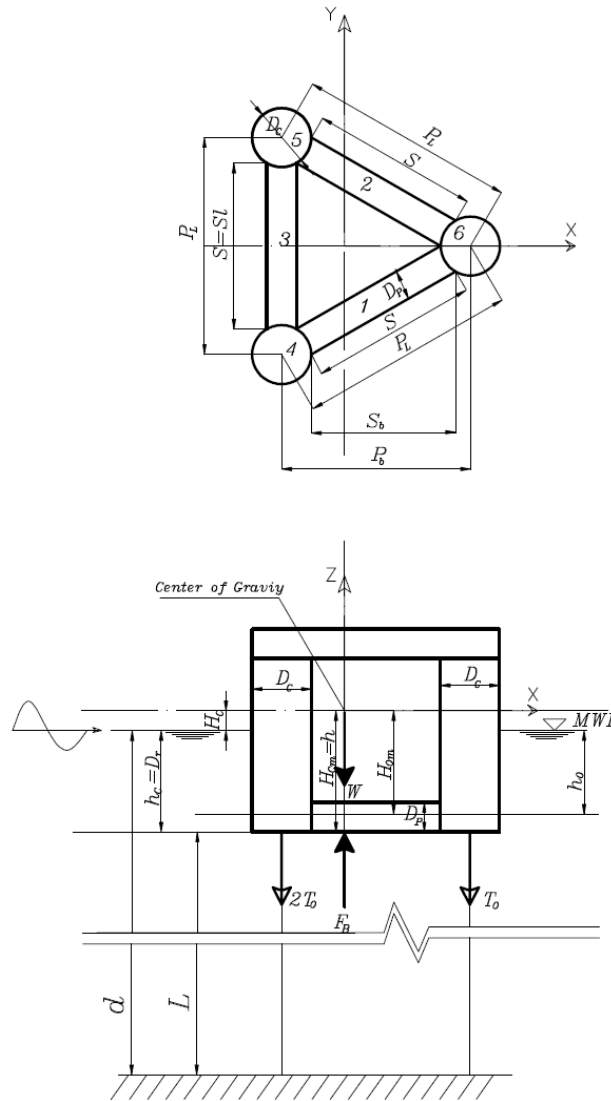
Fig. 1 The Triangular TLP (plan and elevation)
