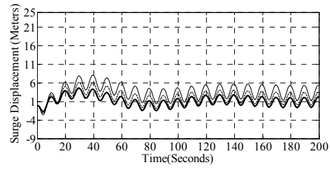
(c) wave period = 10 sec
