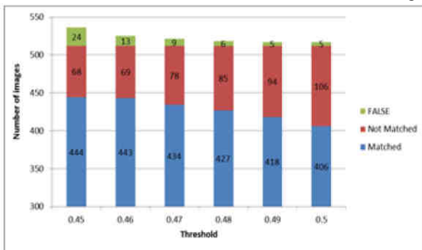
“Fig.7” Results of Matched, Not matched and False fingerprint images when using Huffman compression technique at different thresholds
